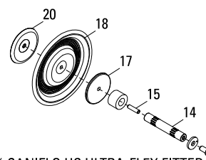
SD1 1/2 SANIFLO HS ULTRA-FLEX FITTED
