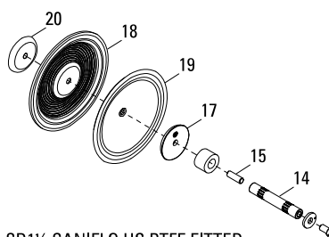
SD1 1/2 SANIFLO HS PTFE FITTED
