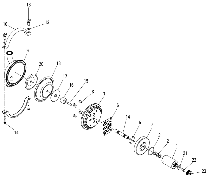
SD1 1/2 SANIFLO HS RUBBER FITTED
