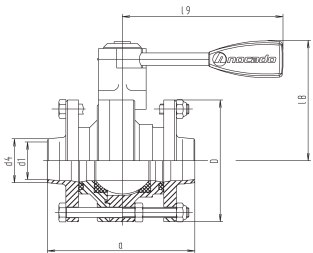
ball valve, betw. flanges, inch OD (860Z)
