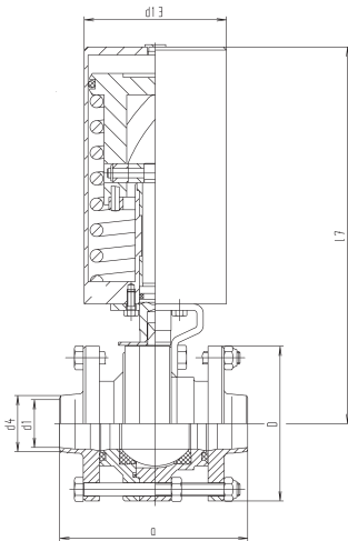
ball valve, betw. flanges, air/spring (NC), inch OD (860)
